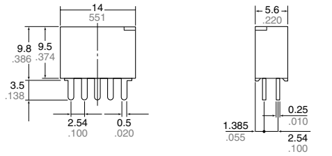
Self-clinching terminal
