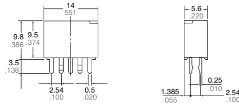
Self-clinching terminal
